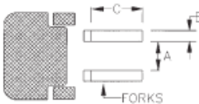
COUNTER BALANCE TRUCK (N)
