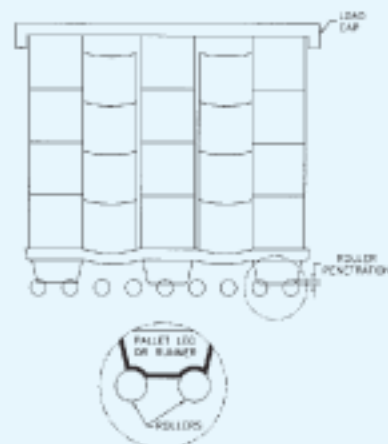
CONVEYOR ROLLER LOAD (DEFINITION ENHANCED)
